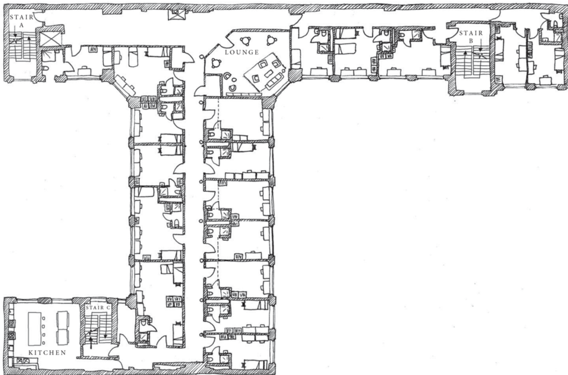
G.27 TYPICAL RESIDENTIAL LEVEL PLAN
